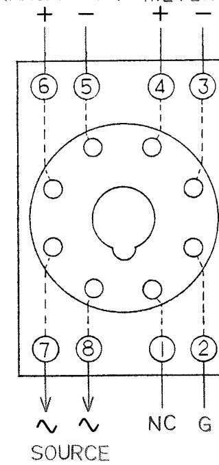
CONNECTION DIAGRAM 2 WIRE TRANSMITTER METER
