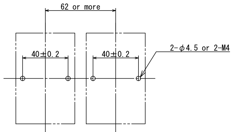
INSTALLATION MEASURE DRAWING (取付寸法図)
